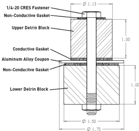
Figure 2-1 Test Fixture
