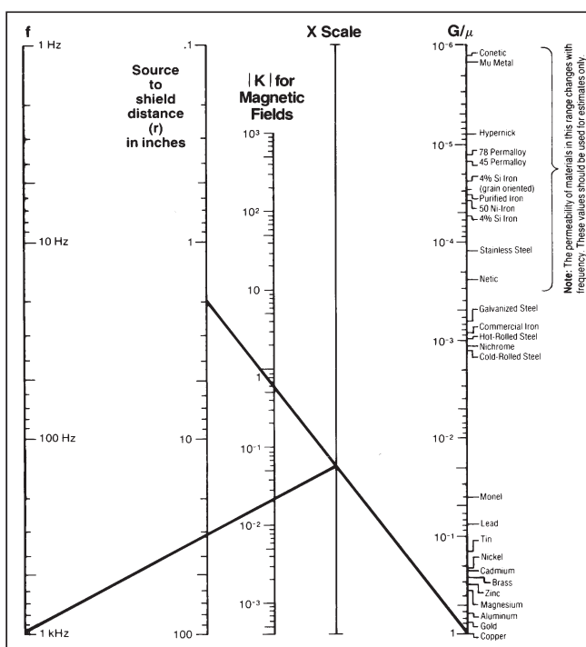
Figure 1-7 Magnetic Field Secondary Reflection Factor Nomograph 1
