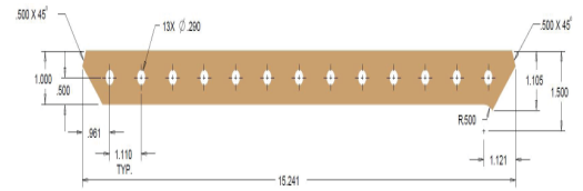
Figure 4-9 - TP09 Plastic Compression Stop.
