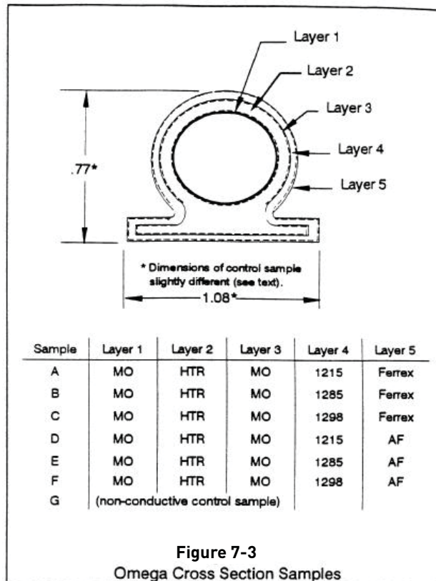
Omega Cross Section Samples
