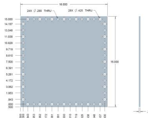
Figure 4-8. CHO-TP09 Aluminum Cover.
