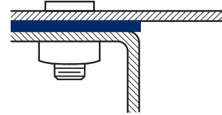
Figure 3-7. Insert Pressed-In and Flared Makes EMI Tight Joint (Alternate: Weld or Cement with Conductive Epoxy)
